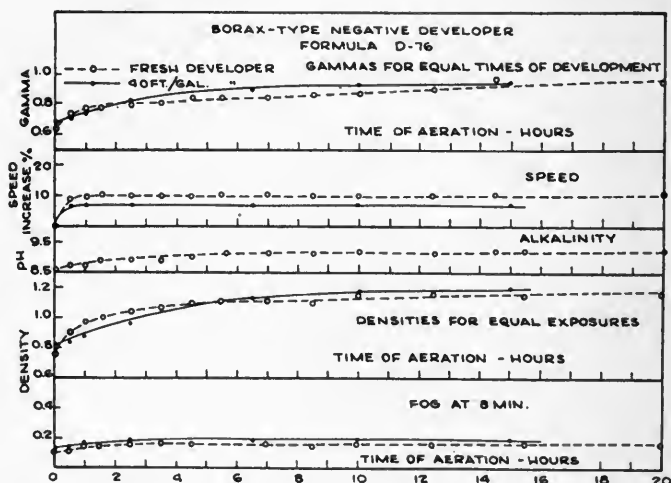
FIG. 2. Effect of aeration of a borax-type of negative developer (Formula D-76).
